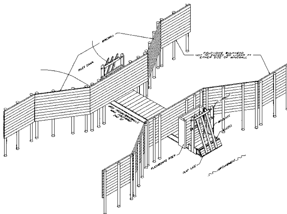
Typical Combahee style rice trunk water control structure. Ducks Unlimited
